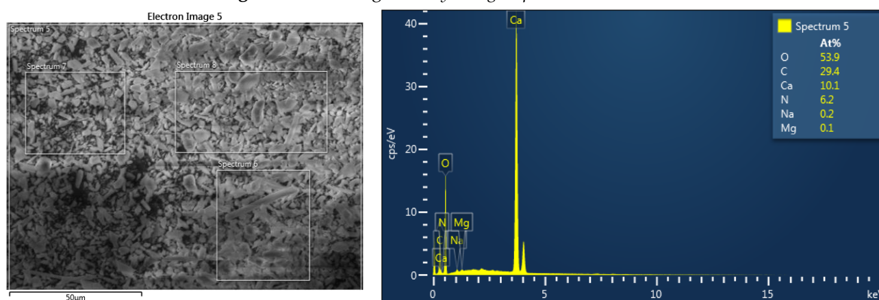
Figure 2. SEM images of Mytilus galloprovincialis shells
